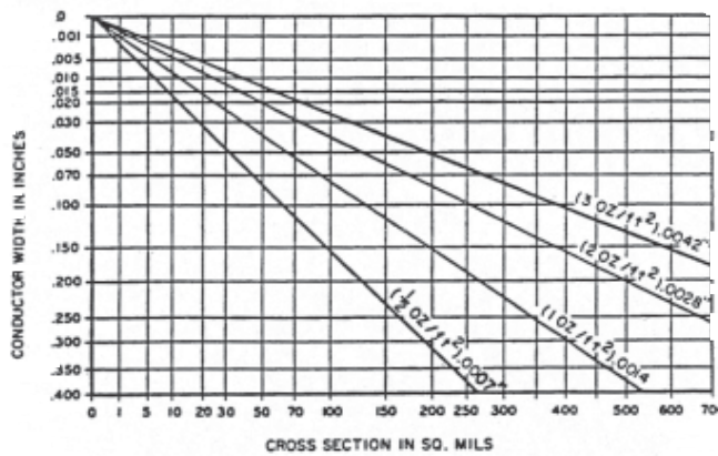
Figure B Conductor width to cross-section relationship
