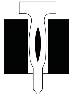
Drill hole size of 1.15 mm -03 , 25-50 µm Cu, and 5-15 µm Sn.
